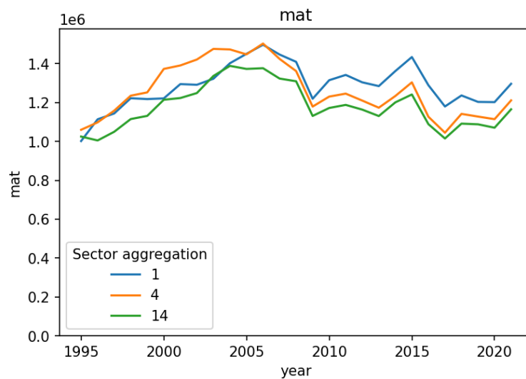
Figure 1. The UK's total material footprint from EXIOBASE.
