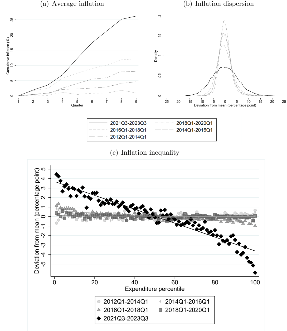
Figure 1: Household-level inflation
