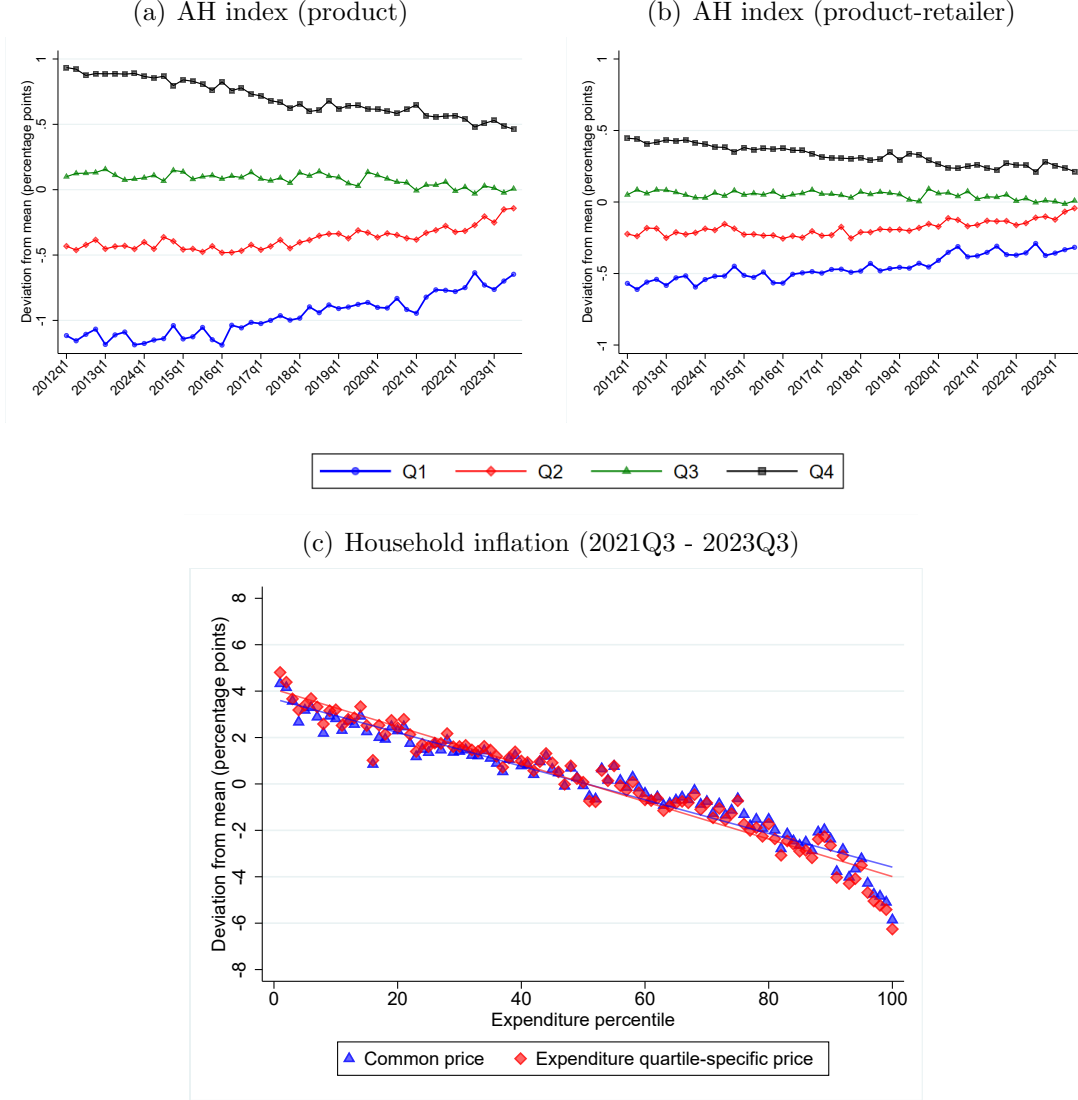
Figure 2: Price dispersion
