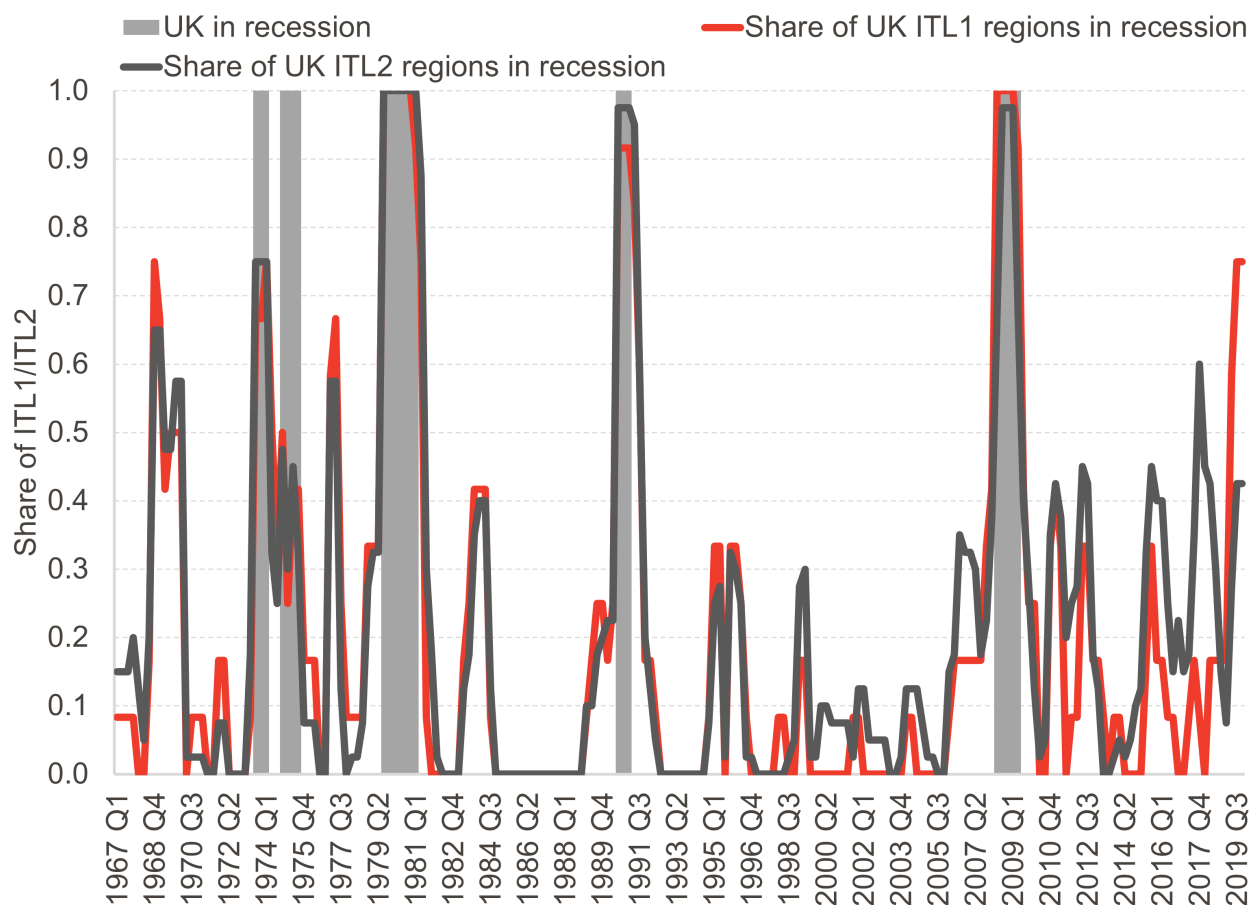
Figure 3: UK recession bands (vertical grey bars) alongside the share (proportion) of regions (ITL1) and sub-regions (ITL2) in (local) recession
