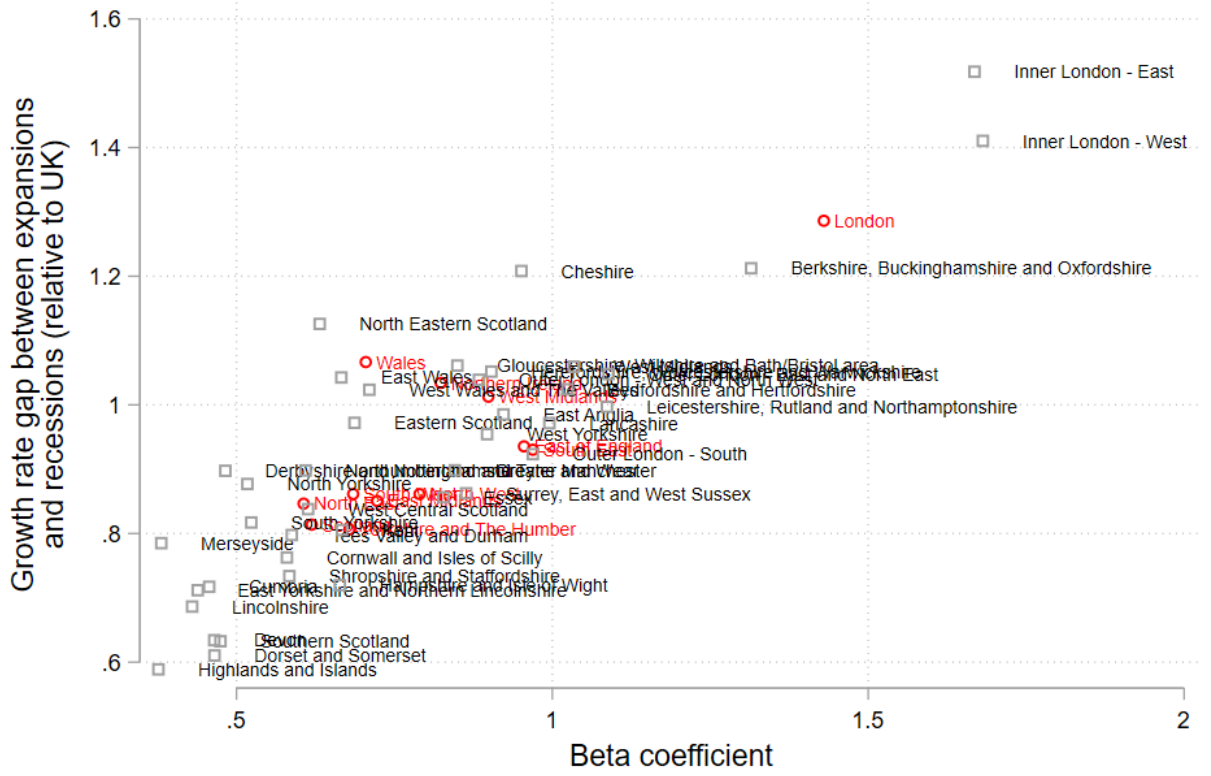
Figure 5: Relative depth of (sub-)regional business cycles (sub-regional average growth rate in expansions minus recessions) versus estimates of \beta (the sensitivity of each sub-region to the UK, as estimated via (12))
